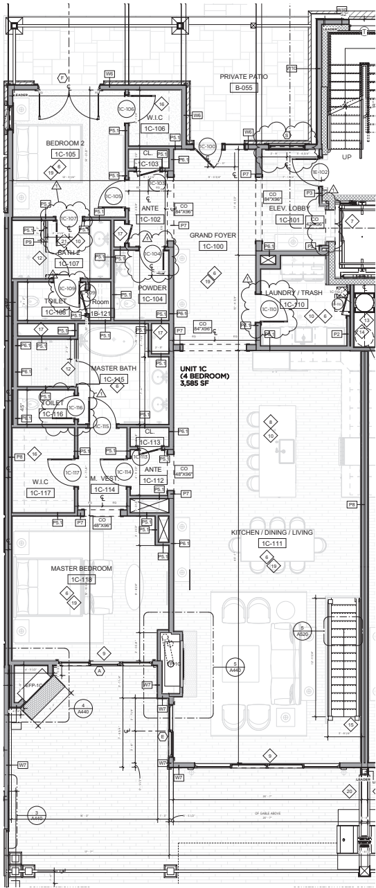
UPPER LEVEL
