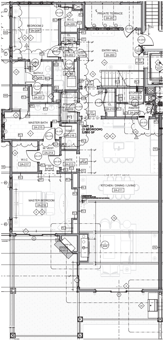
LOWER LEVEL
