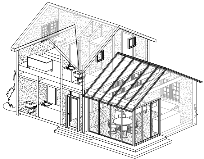
④ TRANSPARENT VIEW
